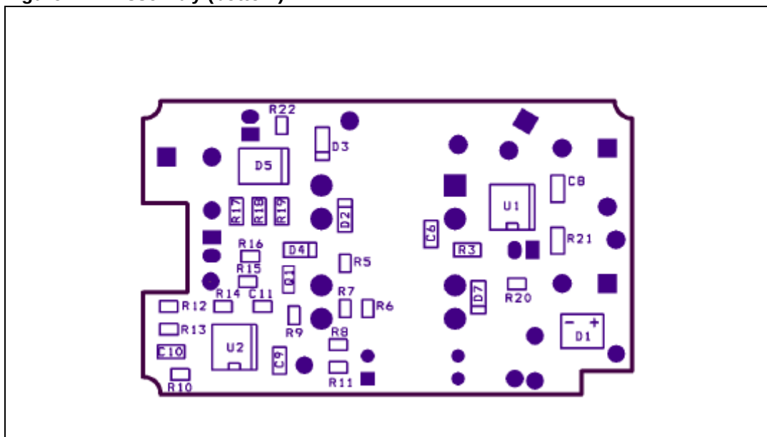
Figure 4. Assembly (bottom)
